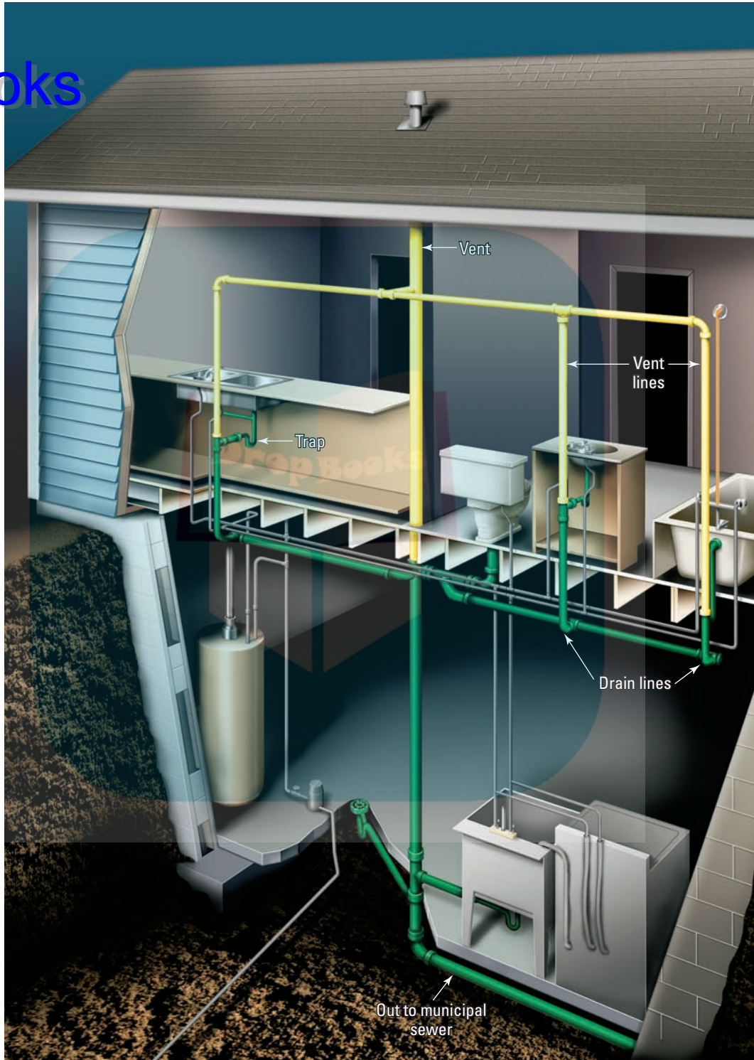
Figure 1-3: The DWV system.
